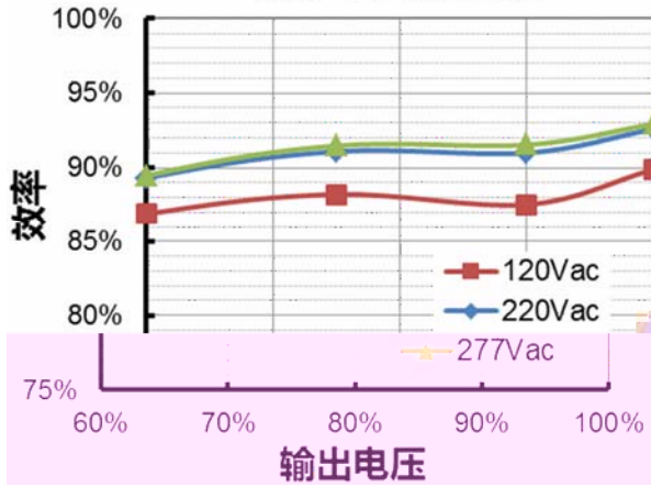
EUP-320S670ST (Io=4690mA) 效率 vs. 输出电压
